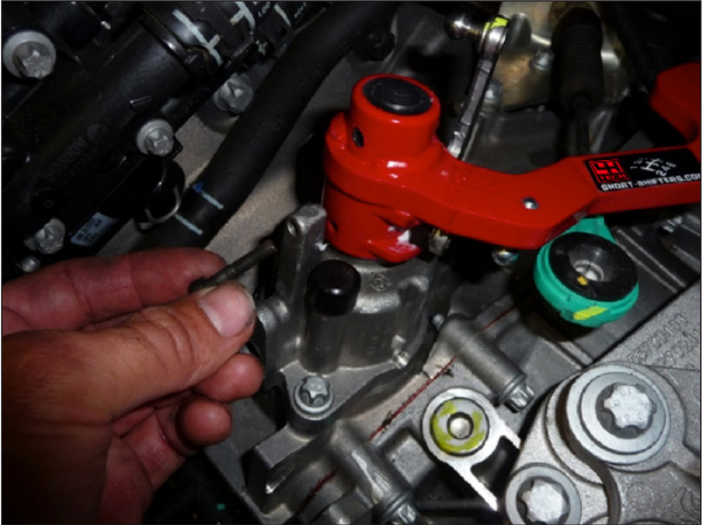
Fit 2x screw (20Nm / 15lb ft) And remove the locking tool.
